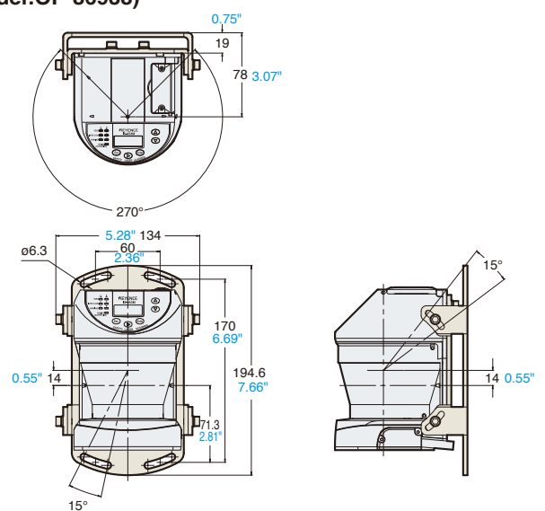
Vertical mounting bracket with angle alignment (Model:OP-86938)
