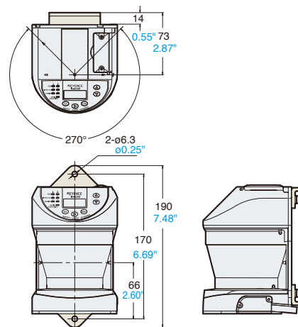
Vertical mounting bracket (Model: OP-86936)
