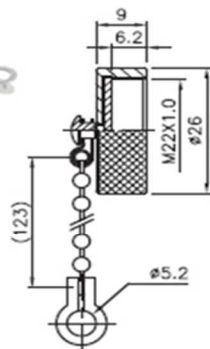
PLS-20-WGPF3 X-R 3=轉接3/8"尼龍管
