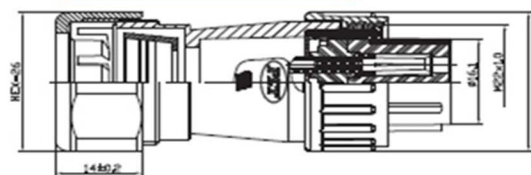
PLS-20-WGPF3 X-R 3=轉接3/8"尼龍管
