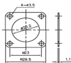
RUBBER PLATE FOR PLS-20-RM
