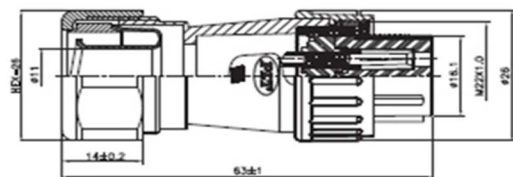
PLS-20-GPF3 X-R 3=轉接3/8"軟管
