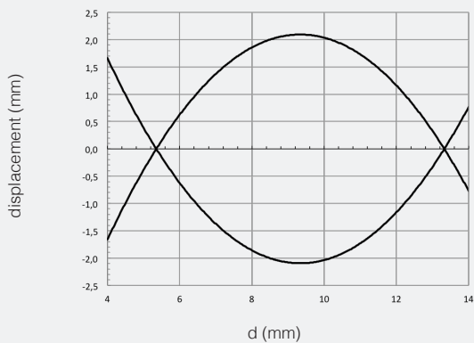
MST/00-**-** + STF12 parallel displacement
