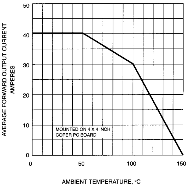
FIG. 2-DERATING CURVE FOR OUTPUT RECTIFIED CURRENT
