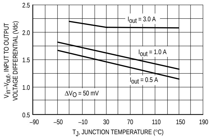
Figure 9. Dropout Voltage
