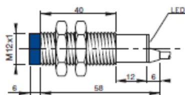
CONFIGURATION WITH CABLE
