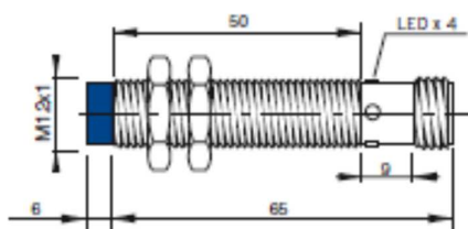
CONFIGURATION WITH CONNECTOR K
