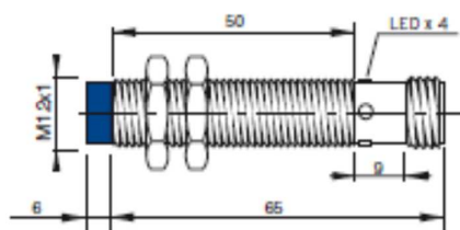
CONFIGURATION WITH CONNECTOR K
