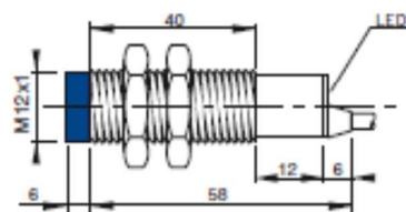
CONFIGURATION WITH CABLE
