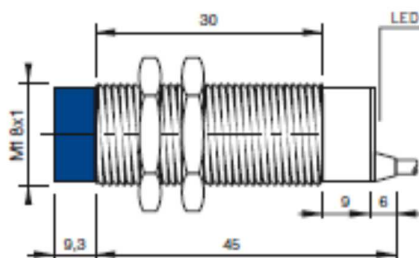
CONFIGURATION WITH CABLE
