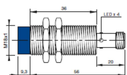
CONFIGURATION WITH CONNECTOR K
