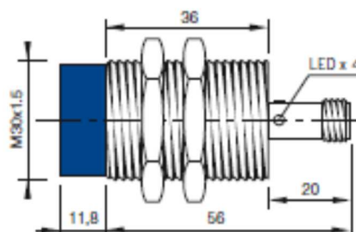
CONFIGURATION WITH CONNECTOR K
