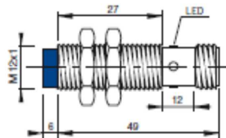
CONNECTOR K
