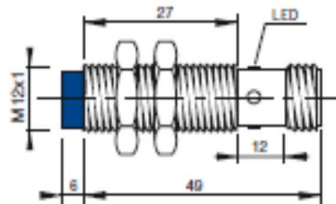
CONNECTOR K
