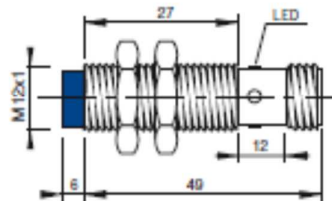
CONNECTOR K
