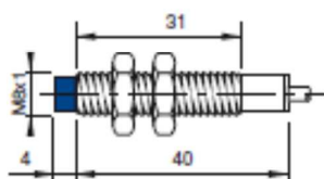
CONFIGURATION WITH CABLE
