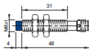
CONFIGURATION WITH CONNECTOR K1
