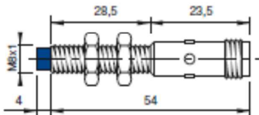
CONFIGURATION WITH CONNECTOR K
