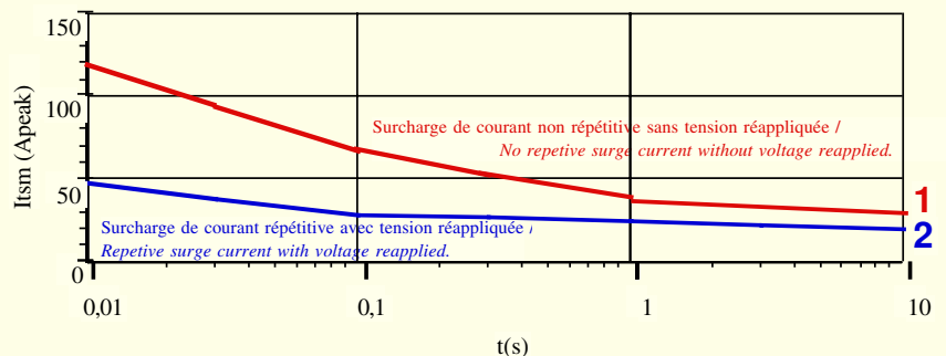
Fig 3 : Surcharge en courant : I_{tsm} (A_{peak}) = f(t) pour modèle 12A ( I_{tsm} = 120A ) / Surge current : I_{tsm} (A_{peak}) = f(t) for 12A models with I_{tsm} = 120A
